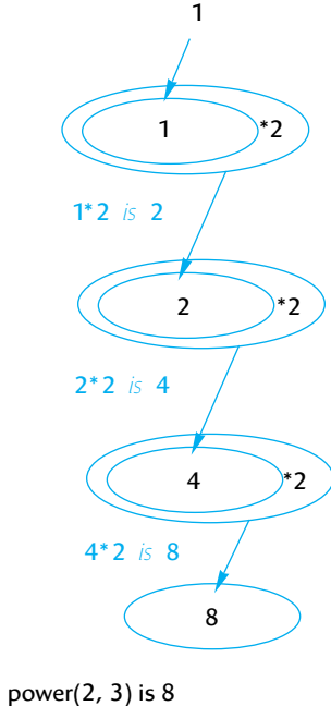
How the final value is computed
