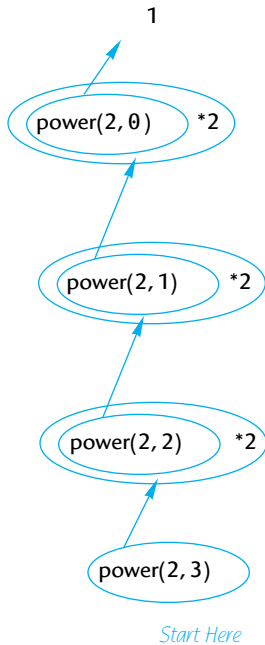
Sequence of recursive calls
